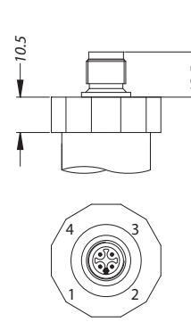
M12x1
