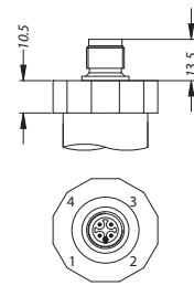
M12x1
